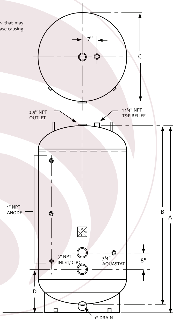
VERTICAL STORAGE TANK
