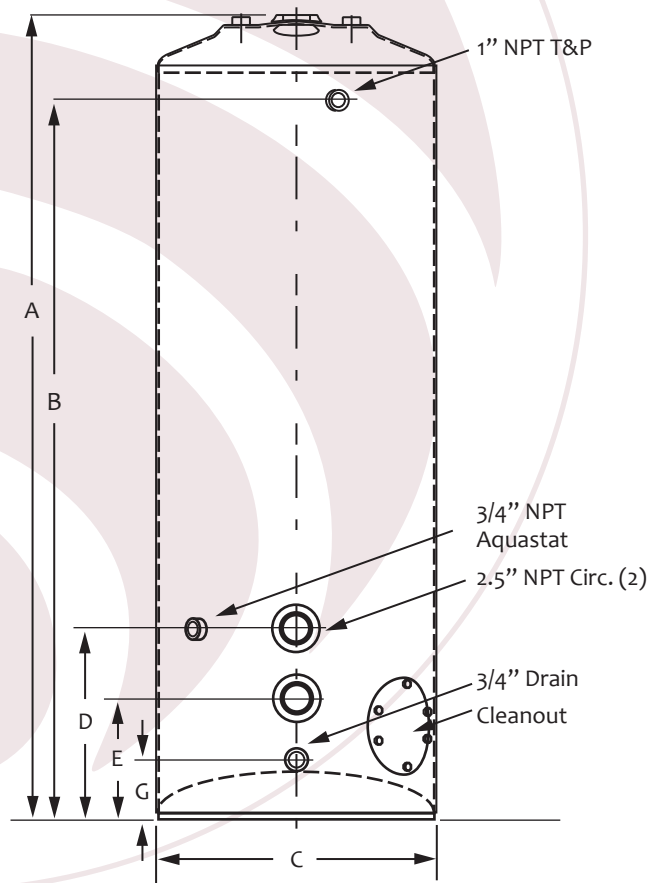
VERTICAL STORAGE TANK
