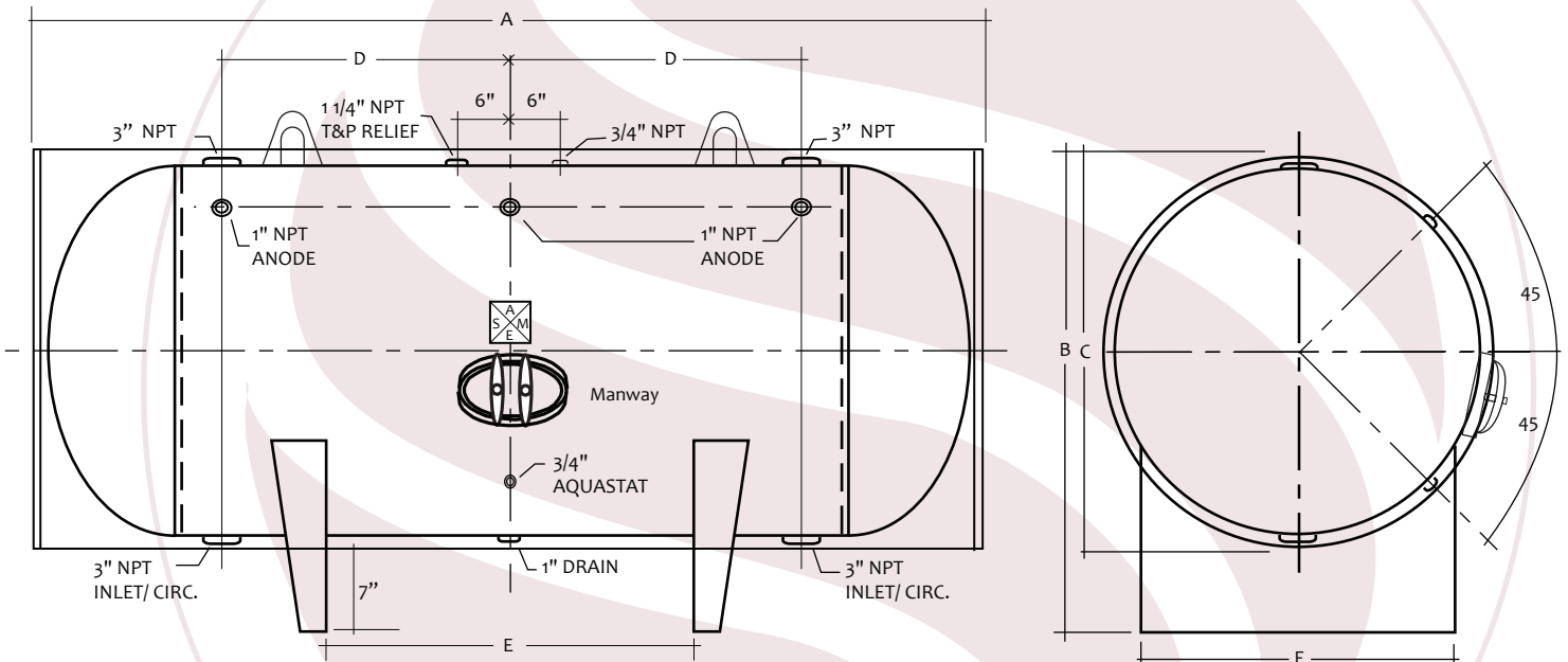
HORIZONTAL STORAGE TANK
