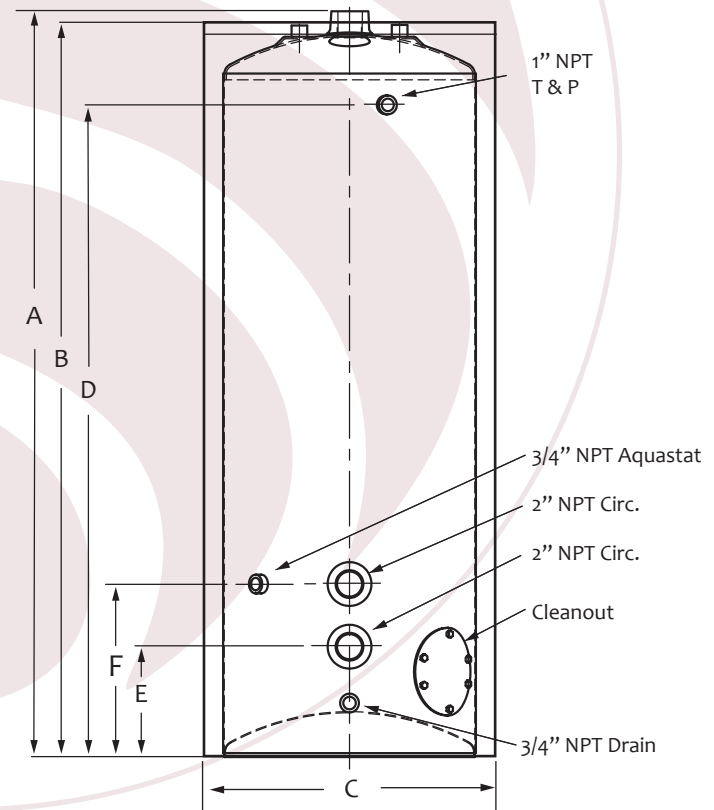
VERTICAL STORAGE TANK
