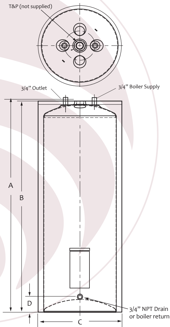
VERTICAL STORAGE TANK
