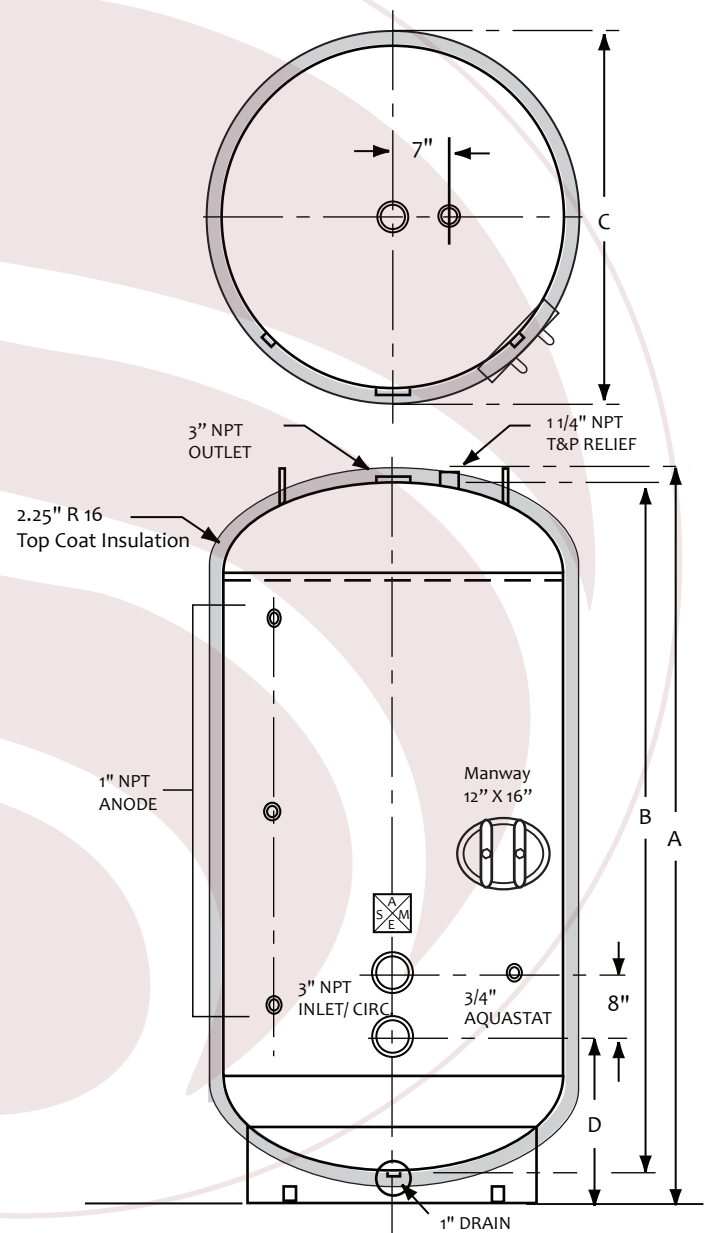
VERTICAL STORAGE TANK w/ topcoat insulation
