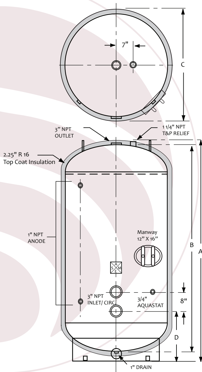
VERTICAL STORAGE TANK w/ topcoat insulation
