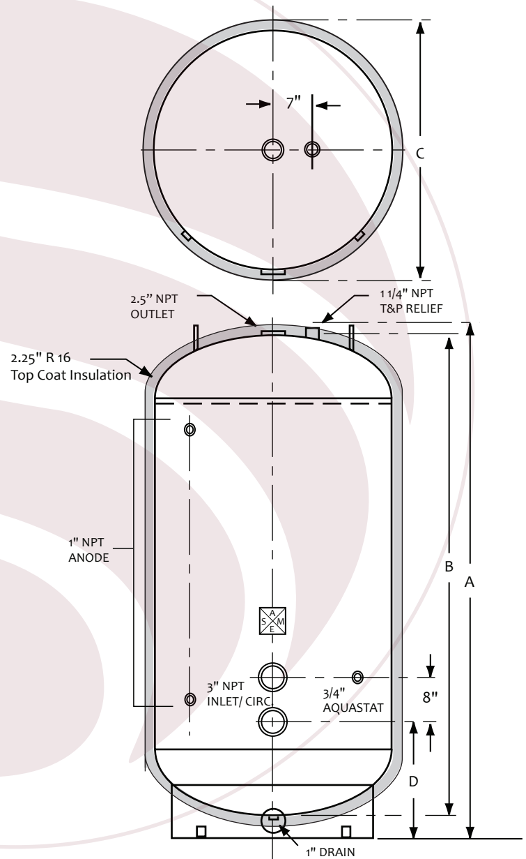
VERTICAL STORAGE TANK w/ topcoat insulation
