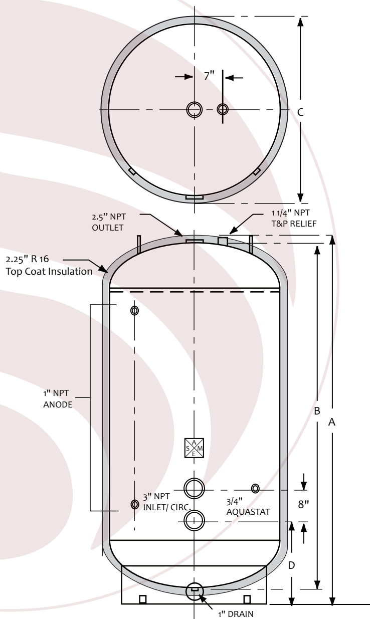
VERTICAL STORAGE TANK w/ topcoat insulation
