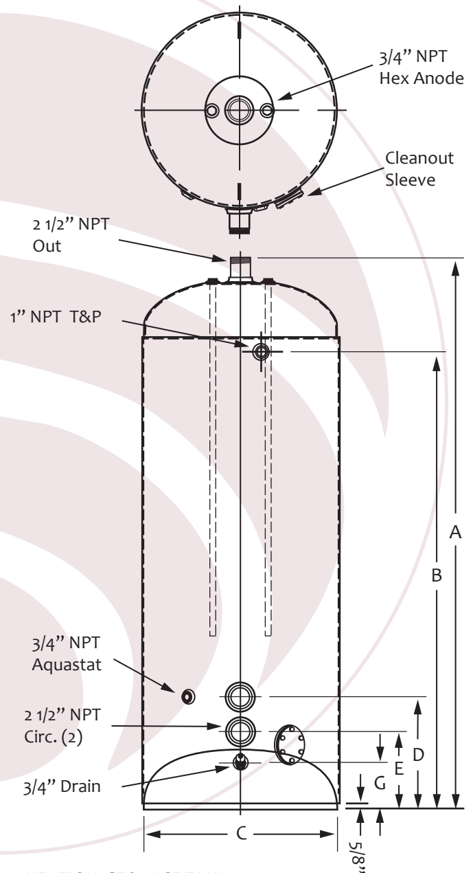
VERTICAL STORAGE TANK
