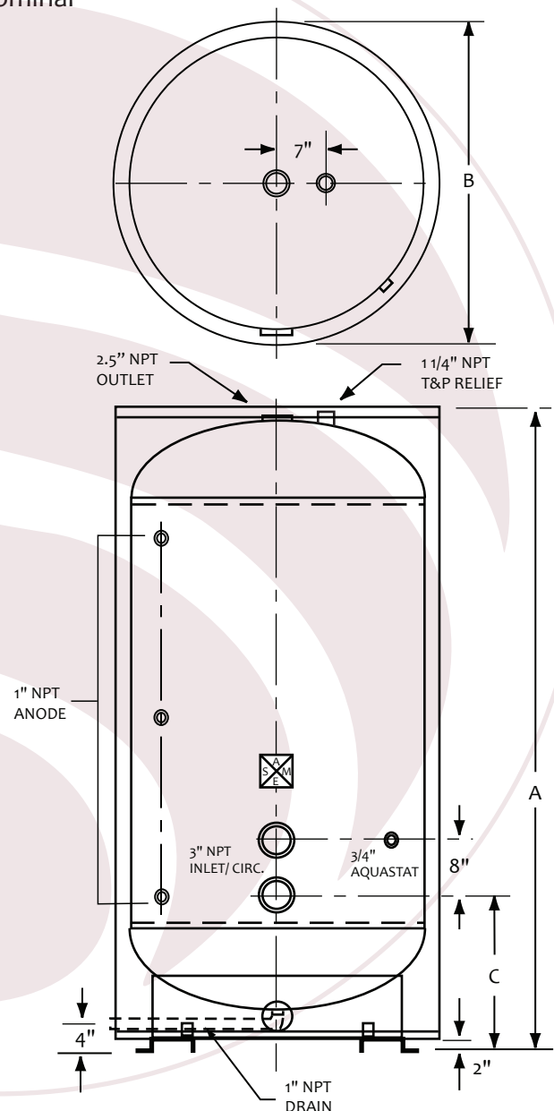
VERTICAL STORAGE TANK
