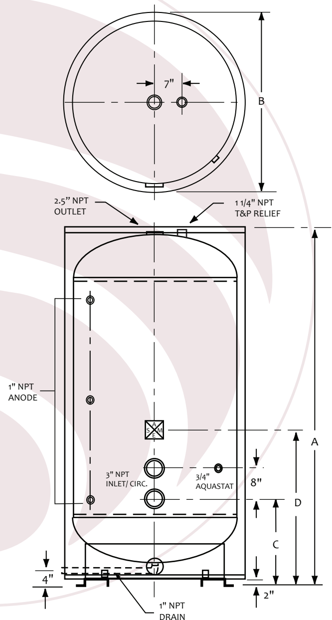
VERTICAL STORAGE TANK
