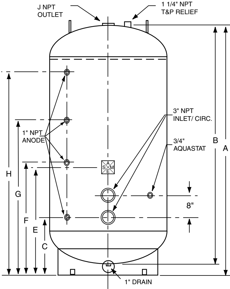
VERTICAL STORAGE TANK
